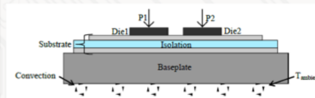
Multichip Module Optimization
